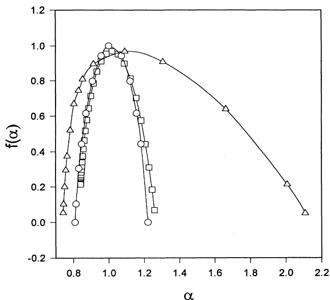
FIG. 1. Multifractal spectra of concanavalin A: \square , spectrum determined from the hydrophilicity profile; \circ , theoretical curve for a multiplicative binomial process used to fit hydrophilicity curve; \triangle , spectrum determined from the solvent accessibility profile.
