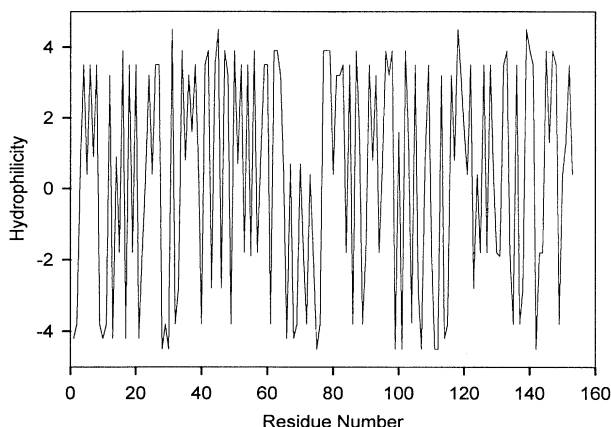
FIG. 2. Hydrophilicity profile of the protein myoglobin (153 amino acid residues). The empirical hydrophilicity index for each amino acid residue is plotted versus the position along the protein sequence.
